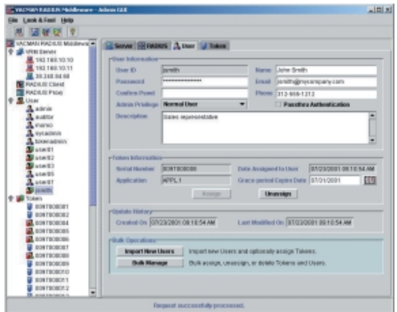
Figure 2: VACMAN Middleware Admin GUI
